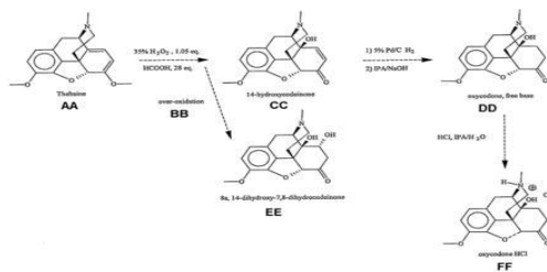
Reaction scheme of the process used to produce oxycodone HCl from thebaine.
